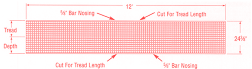
MinTread MS-1515 Molded Stair Treads
