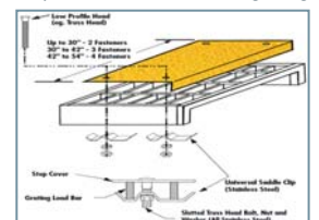
Step Cover installation over grating
