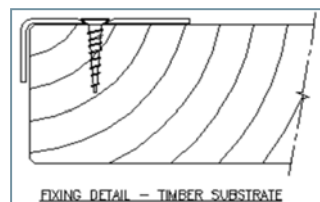
FIXING DETAIL - TIMBER SUBSTRATE
